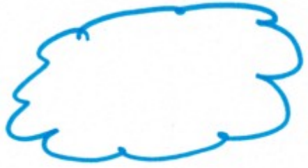
HTTP
